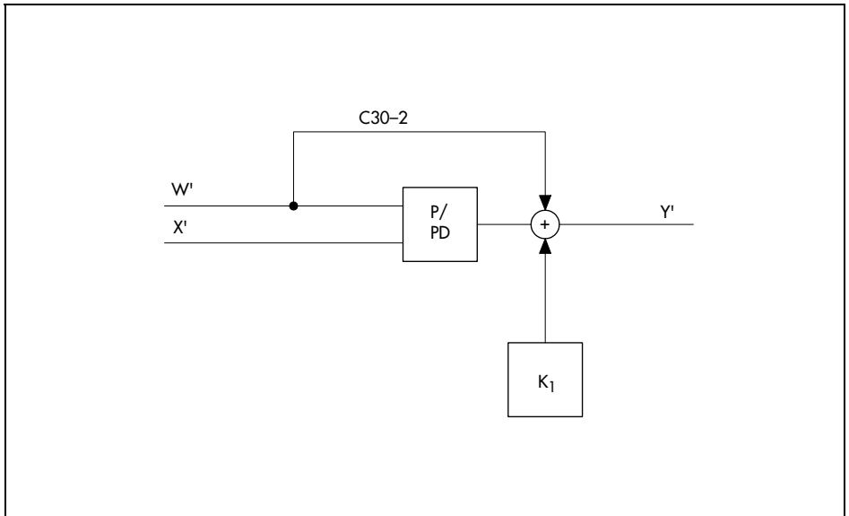
Fig. 69 · Operating point adjustment via reference variable using C30-2
