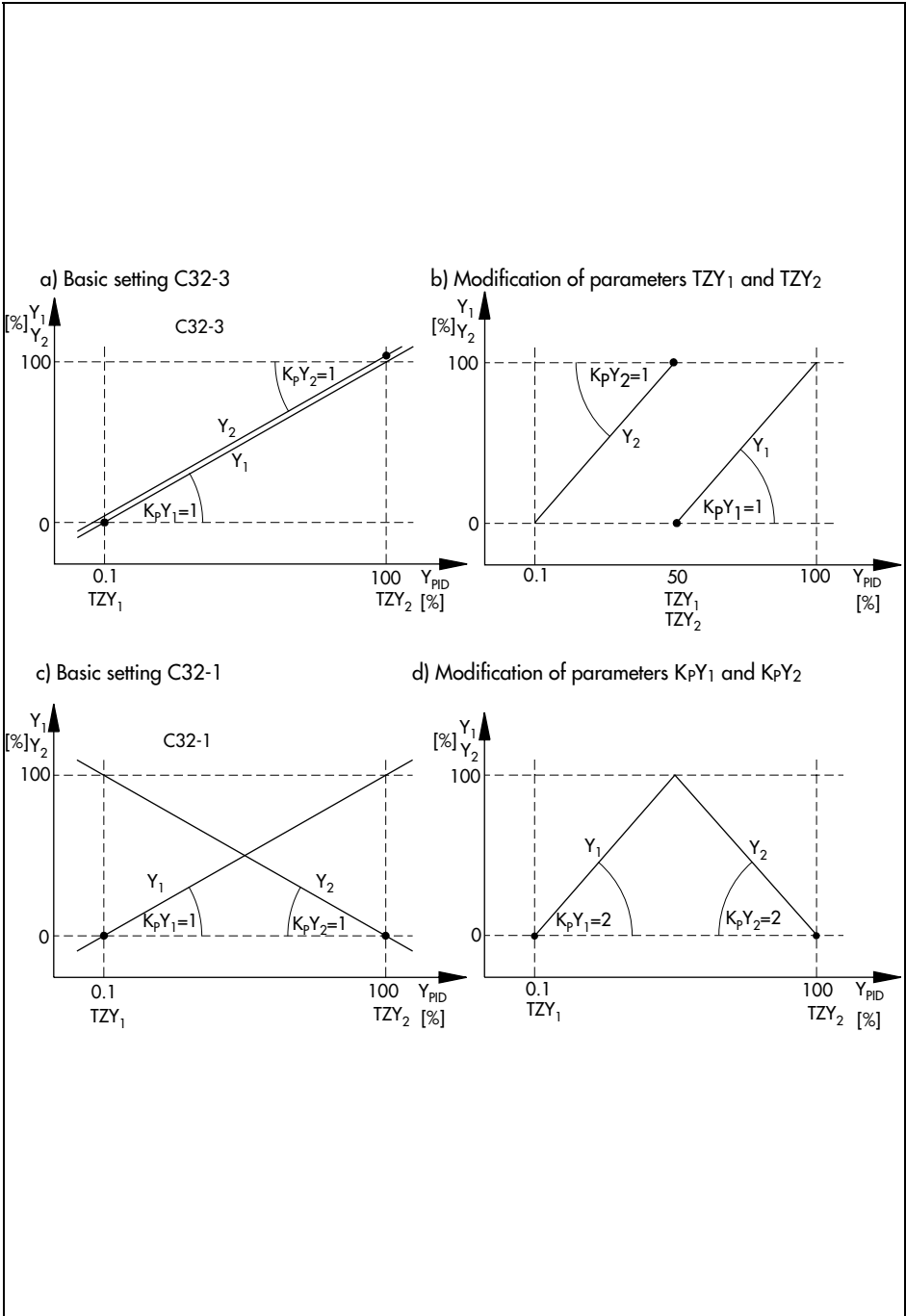
Fig. 50 · Examples for the setting of characteristics
