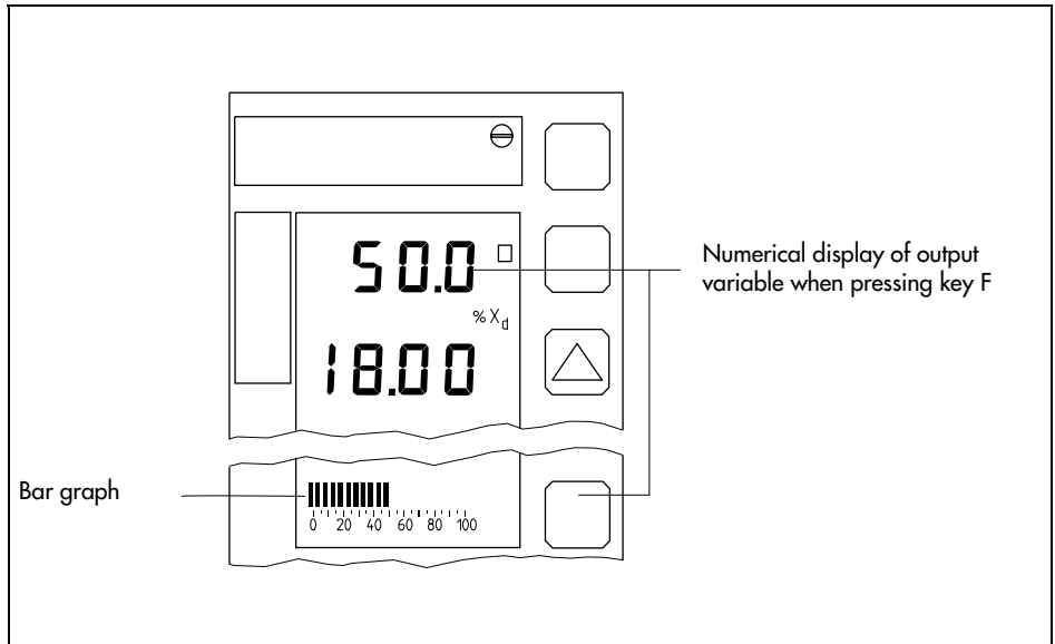
Fig. 79 · Assignment of output variable display
