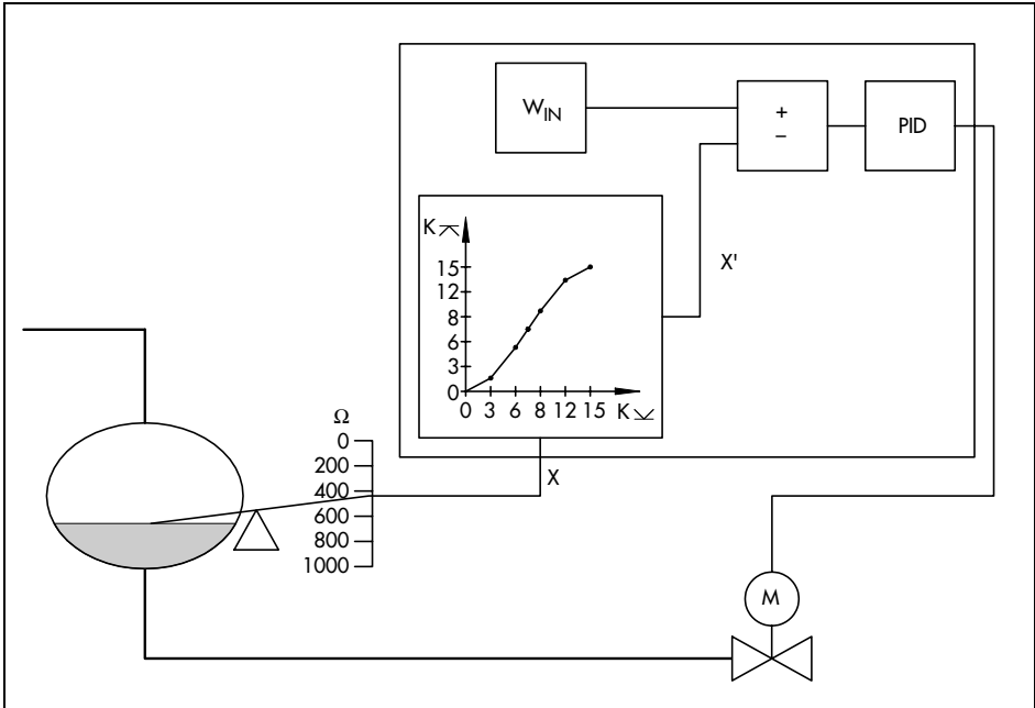
Fig. 9 · Function generation of the liquid level
