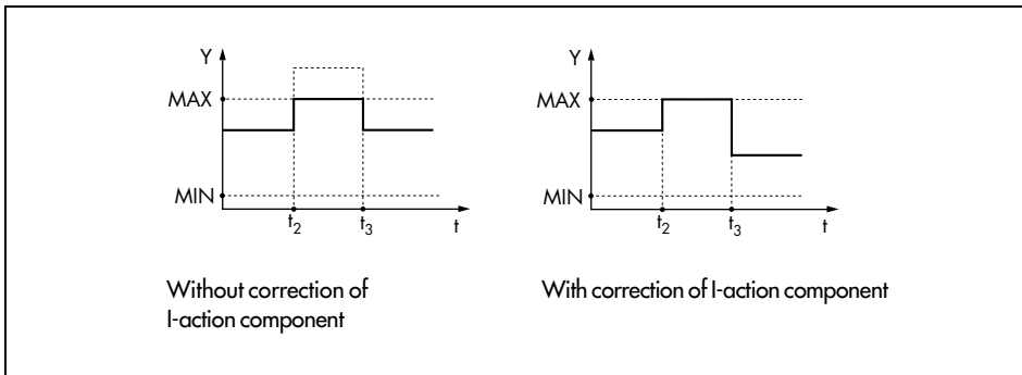
Fig. 65 · Integral-action component correction
