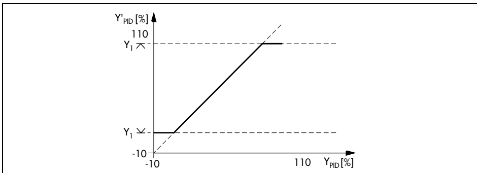
Fig. 51 · Limitation of Y_{PID} via C35-5
