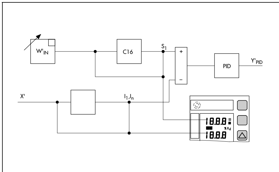
Fig. 74 · Digital displays in fixed set point control mode
