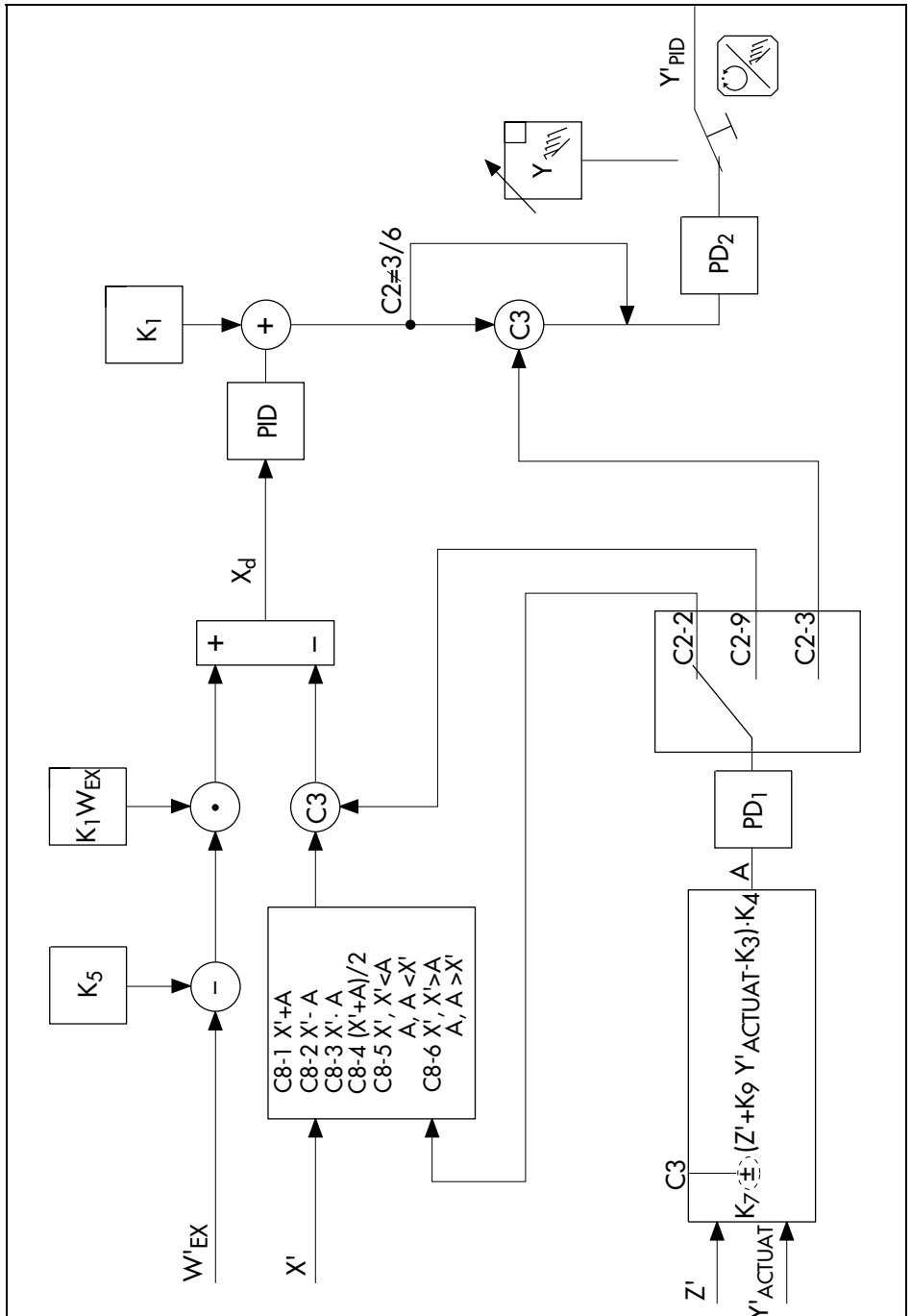
Fig. 41 · Feedforward control for synchro control
