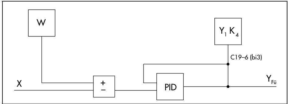
Fig. 16 · Activation of safety output value Y_1K_4
