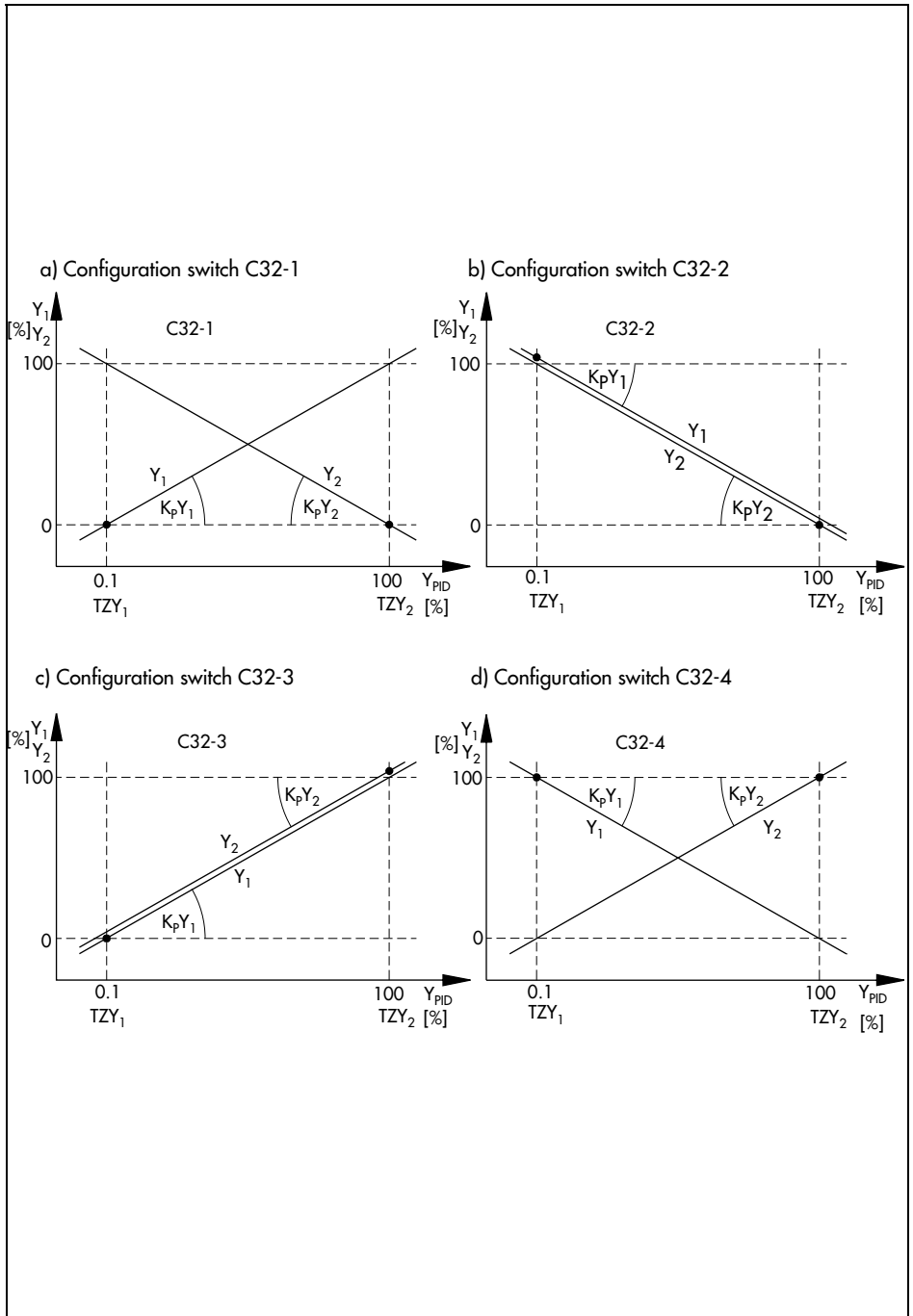
Fig. 49 · Different settings of the operating direction
