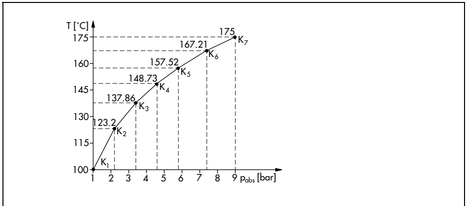
Fig. 7 · Pressure-temperature curve of example 1 for function generation
