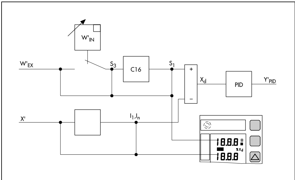
Fig. 75 · Digital displays in follow-up control mode
