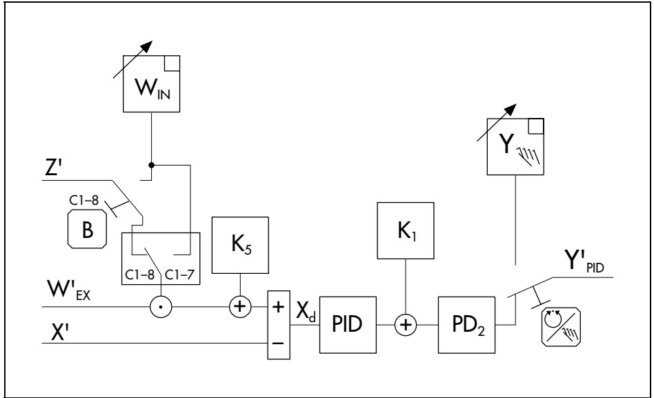
Fig. 25 · Ratio control
