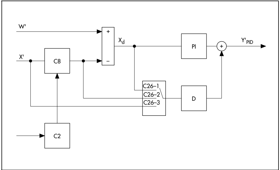
Fig. 66 · Input variable for D element in fixed set point, follow-up, ratio and synchro control mode
