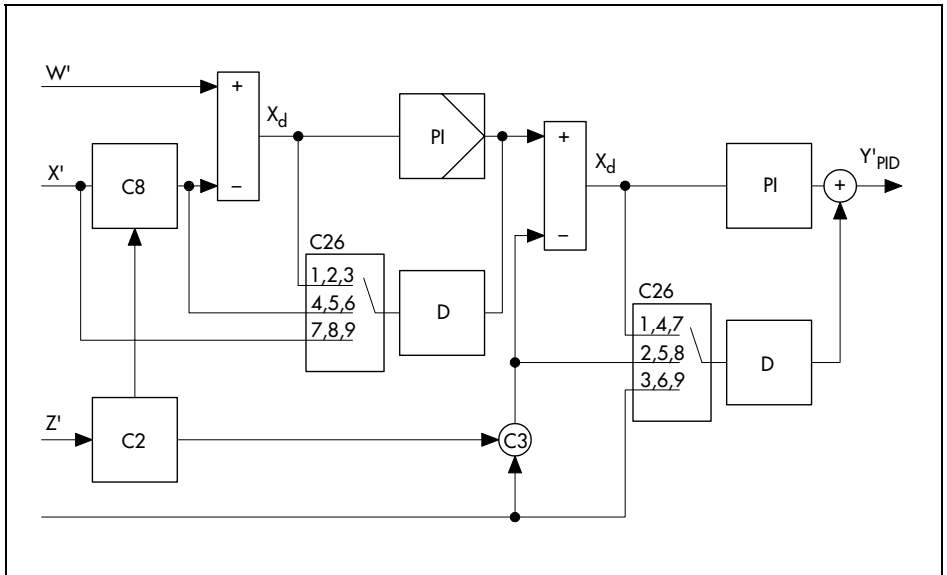
Fig. 67 · Input variable for D element in cascade control mode
