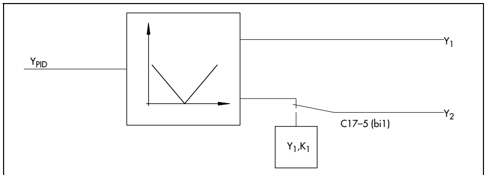
Fig. 13 · Safety output value Y_2K_1 activated by binary input 2
