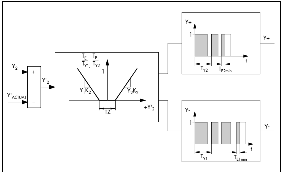
Fig. 47 · Three-step output with external position feedback and PP converter
