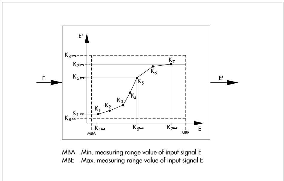
Fig. 6 · Graphical representation of function generation
