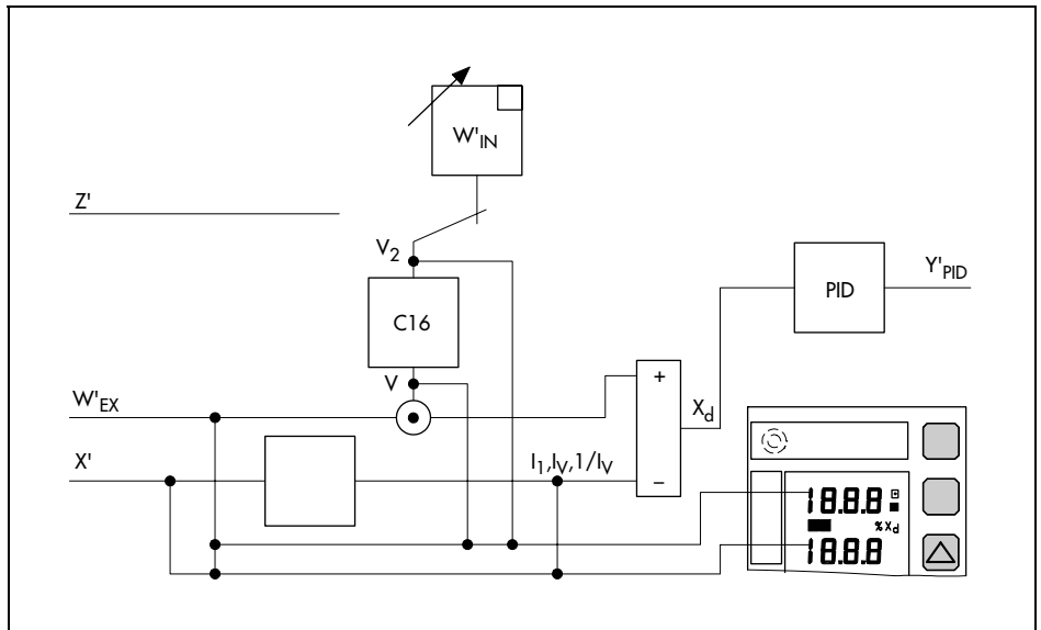
Fig. 76 · Digital displays in ratio control mode
