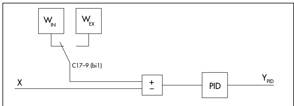
Fig. 19 · Reference variable changeover via binary input 1
