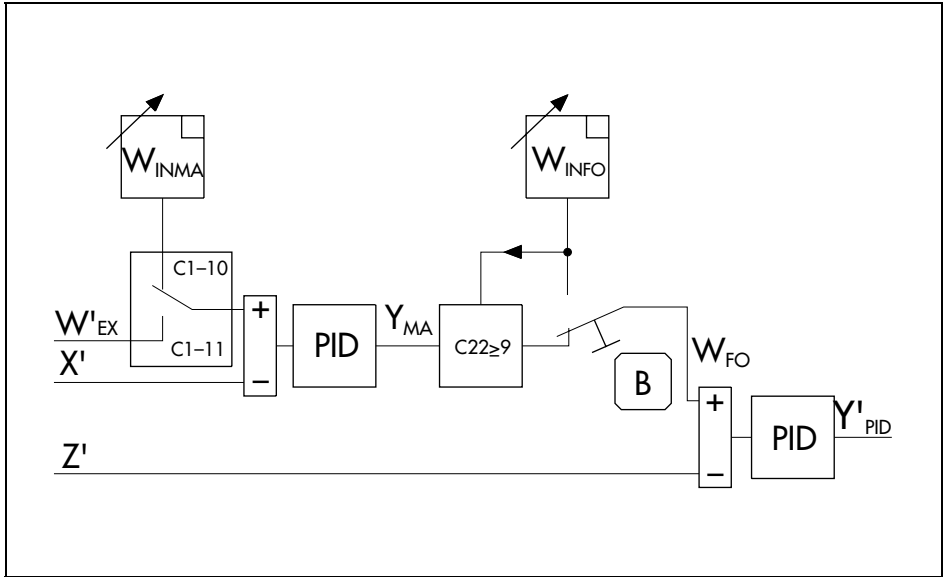
Fig. 27 · Modification of follower controller reference variable for cascade control
