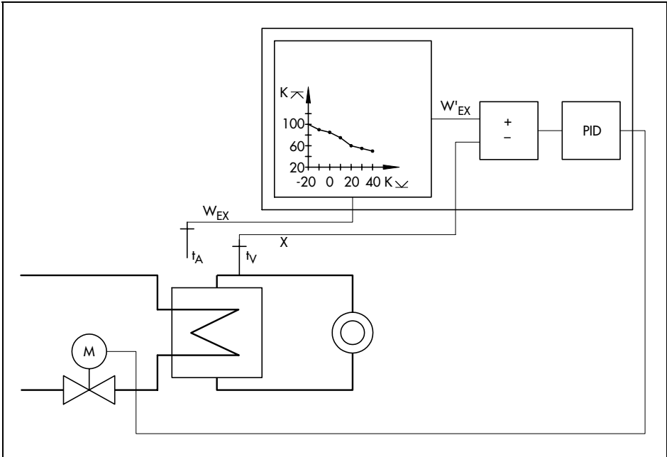
Fig. 10 · Function generation used for weather-sensitive flow temperature control
