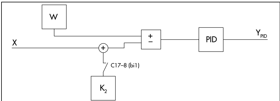
Fig. 18 · Increase or decrease in actual value via binary input 1
