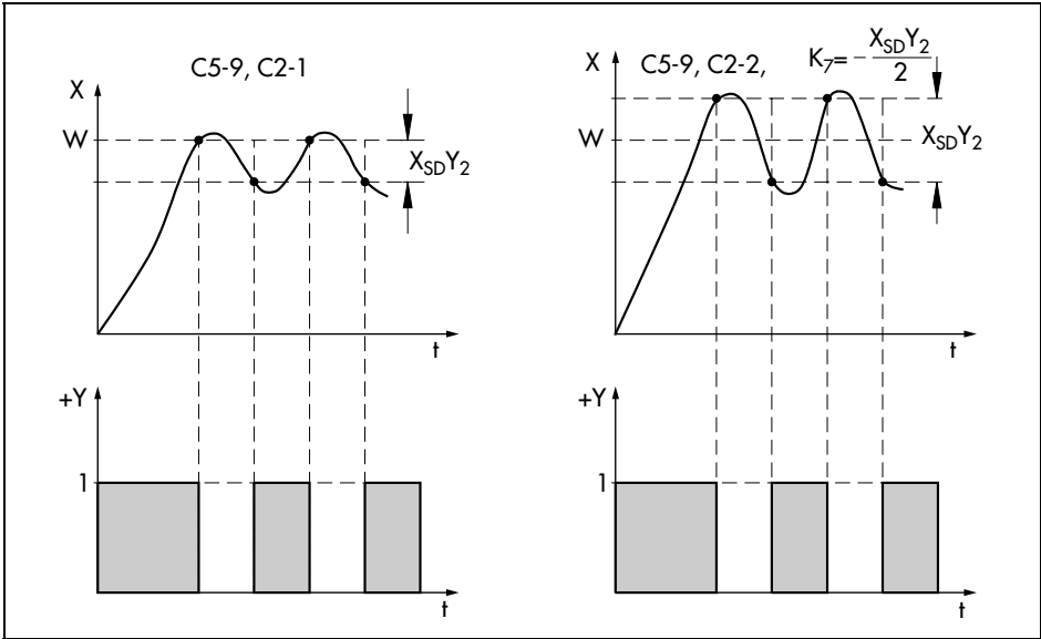
Fig. 43 · Differential gap of on-off output selected via C5-9
