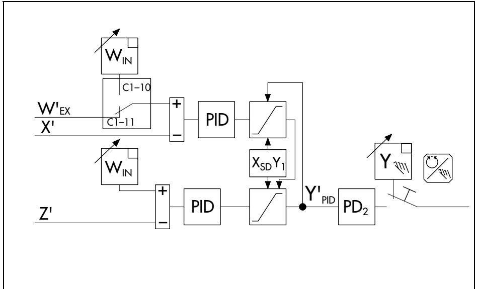
Fig. 29 · Limiting control with selection of either minimum or maximum output variable via C33-14/15
