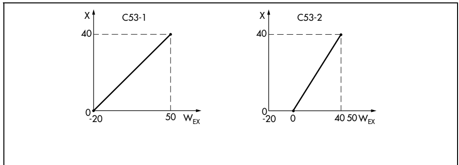
Fig. 73 · Example for measuring range adaptation of W EX input to X input
