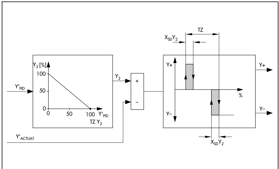
Fig. 45 · Three-step output with external position feedback
