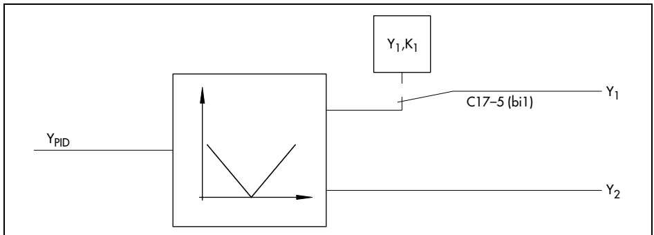
Fig. 12 · Safety output value Y_1K_1 activated by binary input 1
