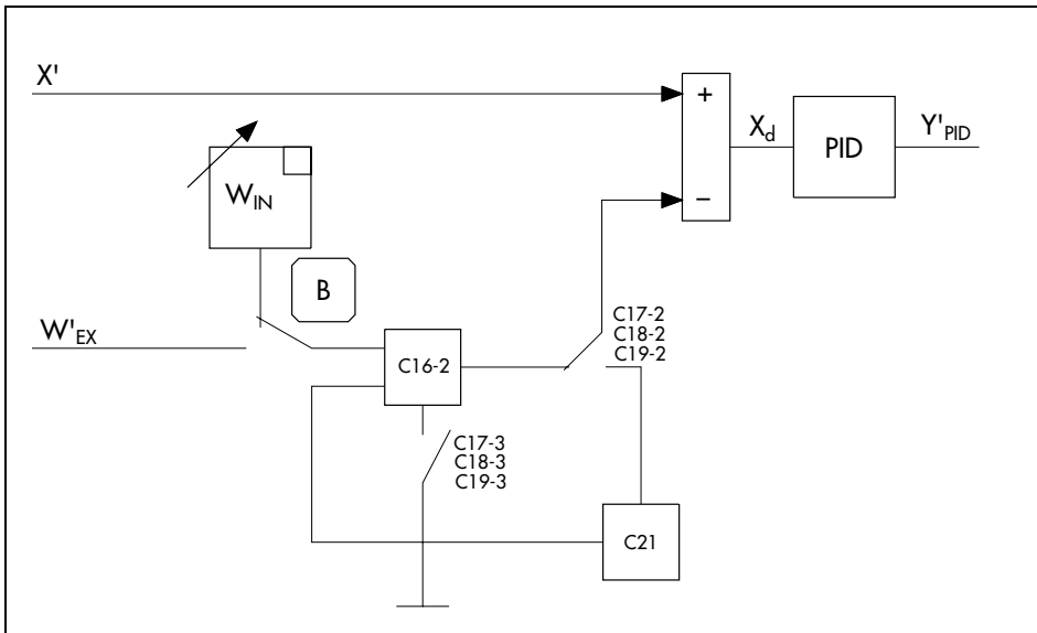
Fig. 54 · Reference variable ramp with starting condition via binary input
