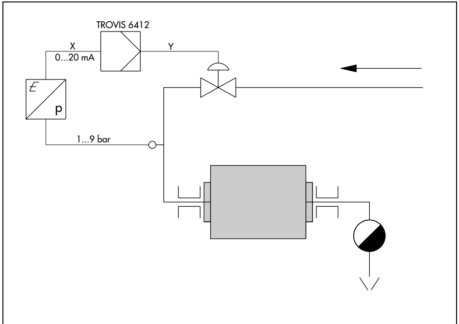
Fig. 8 · Temperature control of a calender bowl
