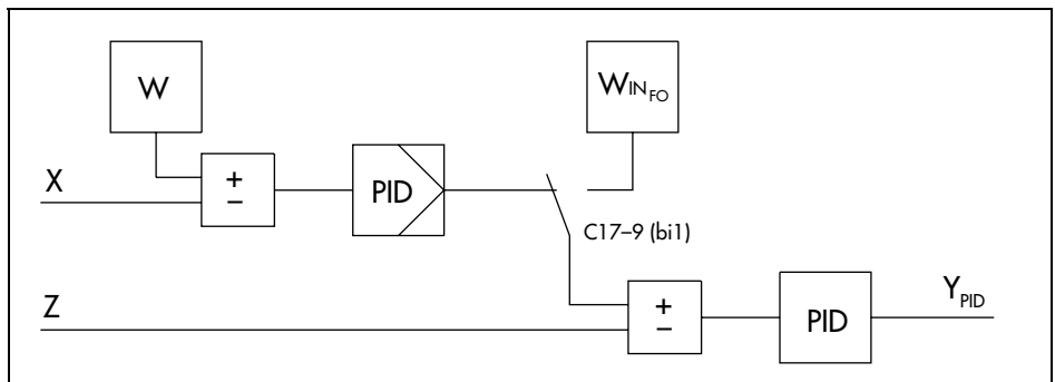
Fig. 20 · Changeover to follower controller mode via binary input 1
