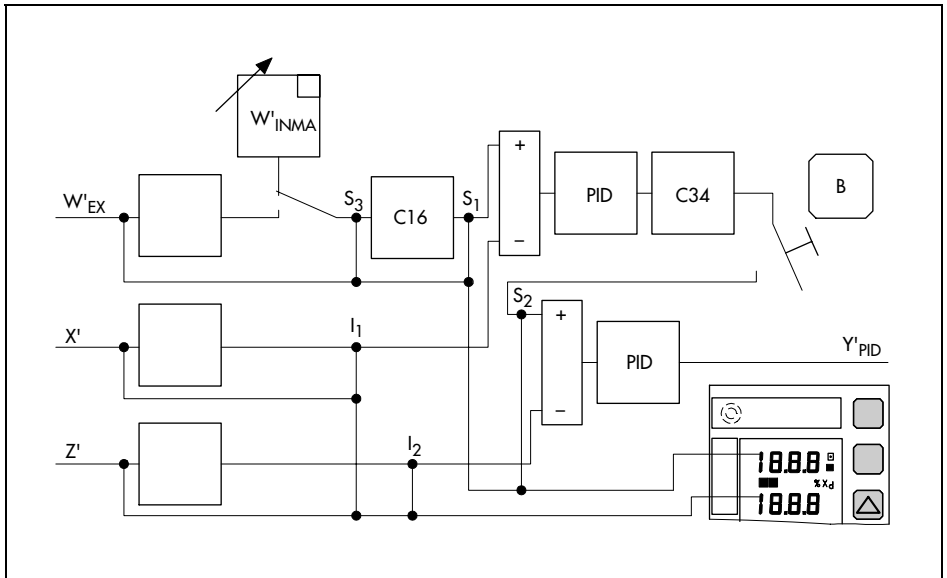
Fig. 77 · Digital displays in cascade control mode
