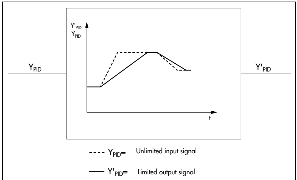
Fig. 58 · Limitation of the rate of output changes via C34-8
