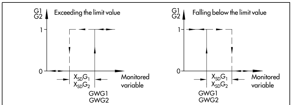
Fig. 52 · Functioning of limit relays G1 and G2
