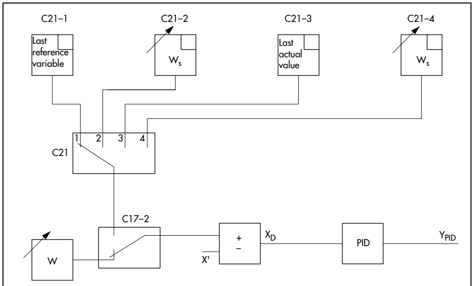
Fig. 11 · Reference variable changeover via binary input
