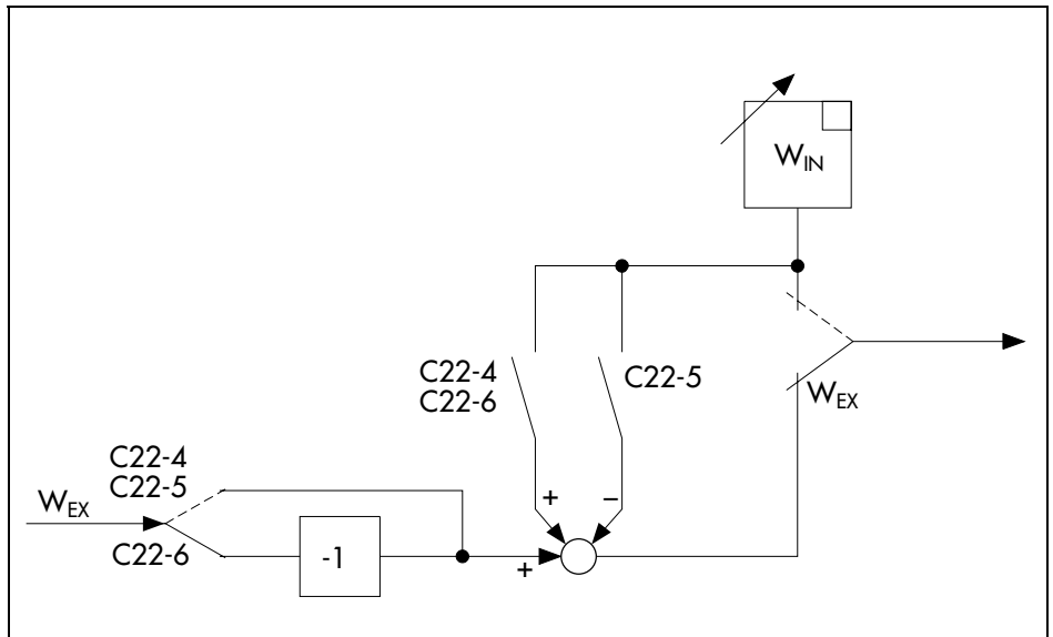
Fig. 59 · Assignment of internal reference variable via C22-4/-5/-6
