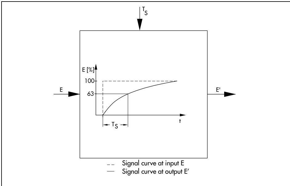
Fig. 3 · Digital filter
