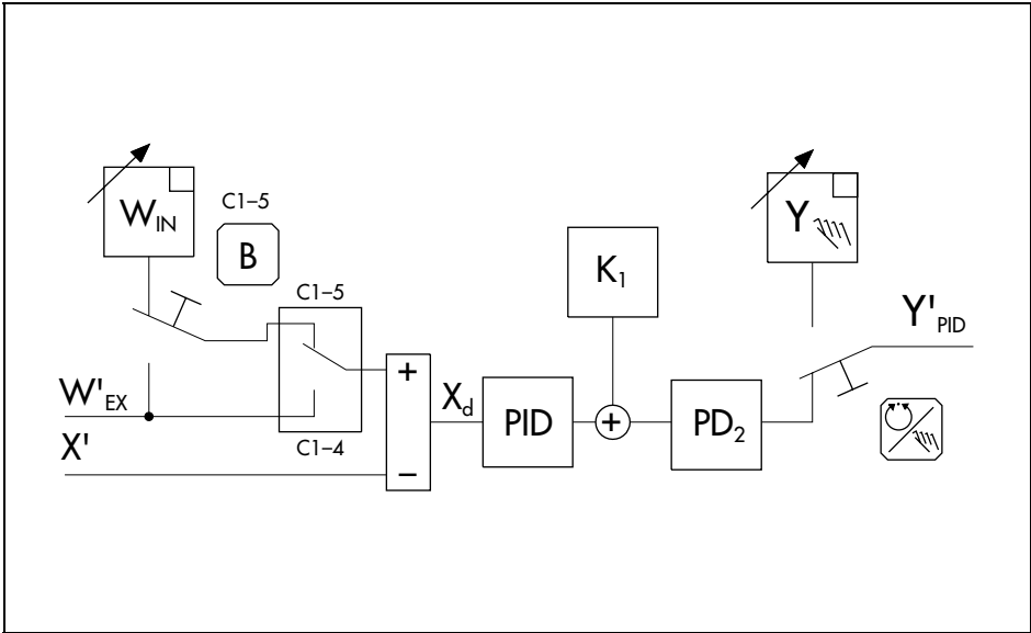
Fig. 24 · Follow-up control
