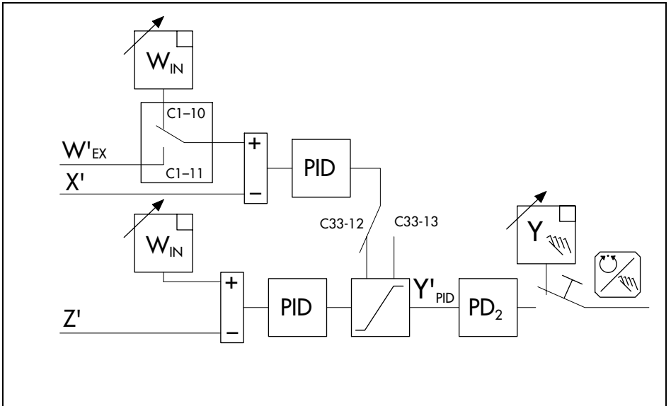
Fig. 28 · Limiting control with limited Y_{PID}
