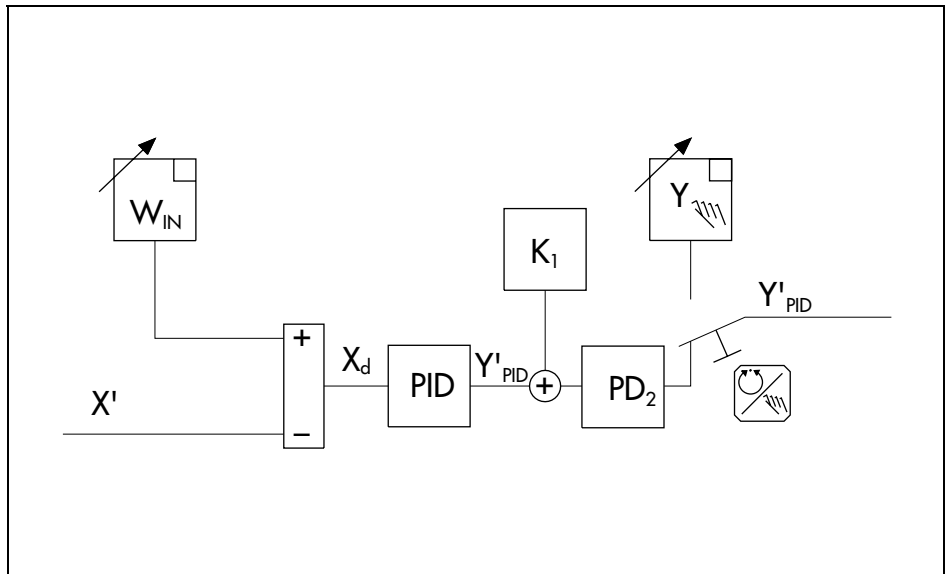
Fig. 23 · Fixed set point control
