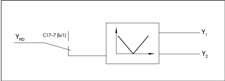
Fig. 17 · Locking of output values Y_1 and Y_2 via binary input 1
