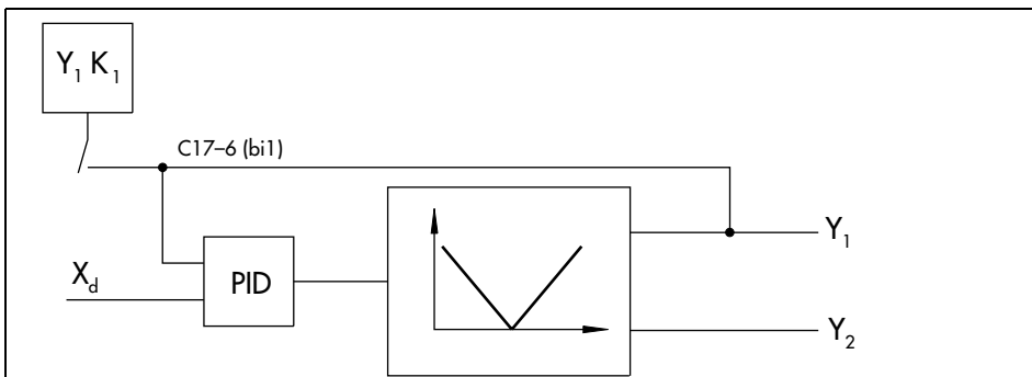
Fig. 15 · Activation of safety output value Y_1K_1 via C17-6 through binary input 1
