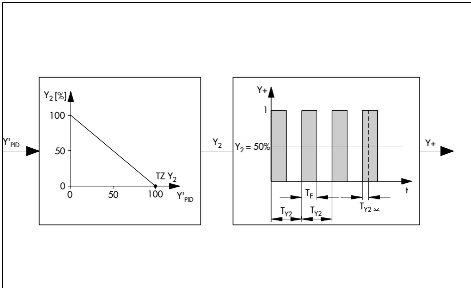
Fig. 44 · On-off output with PP converter
