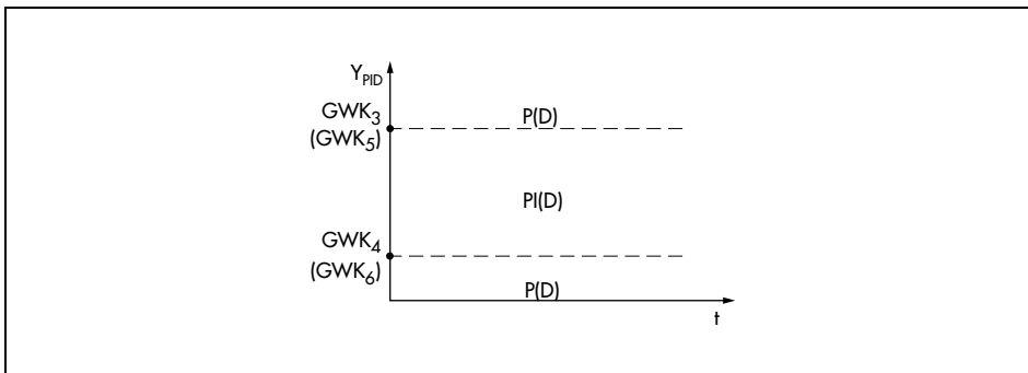
Fig. 70 · Determination of output variable range for P(D)/PI(D) change of control action
