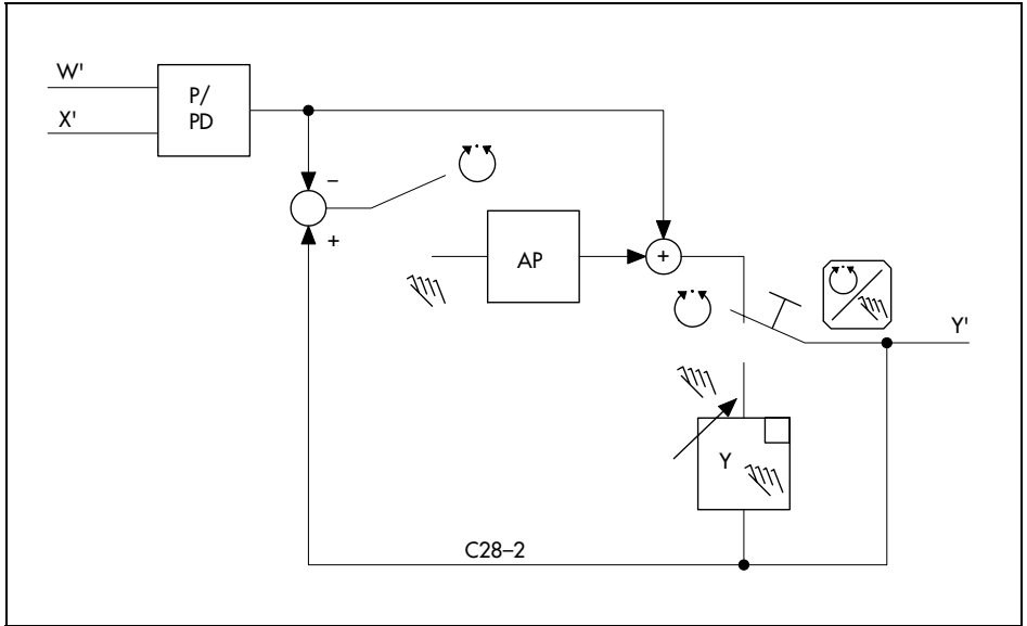
Fig. 68 · Operating point adjustment via manual mode using C28-2
