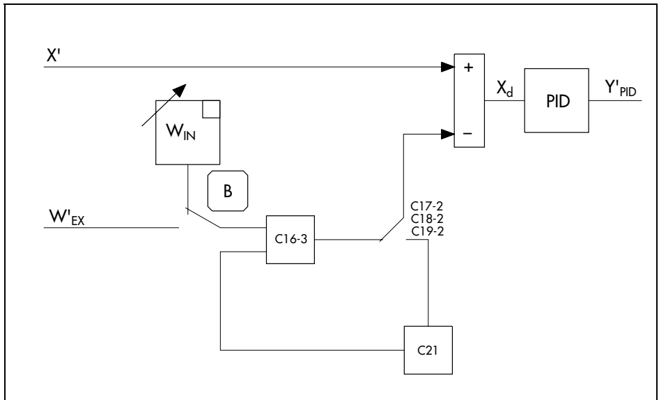
Fig. 55 · Reference variable ramp without starting condition
