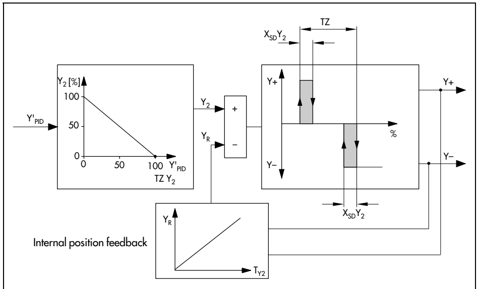
Fig. 46 · Three-step output with internal position feedback
