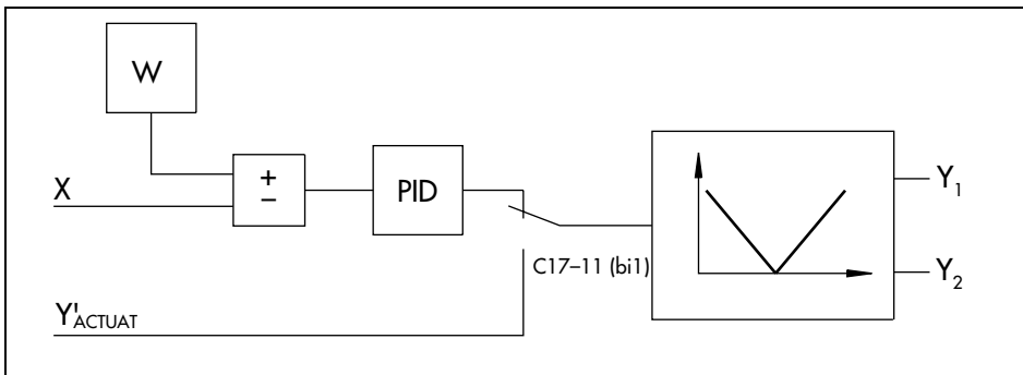
Fig. 21 · Changeover to position correction
