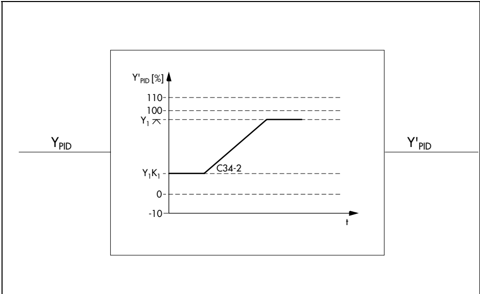
Fig. 57 · Output ramp with starting condition by cancelling the safety mode via C34-2
