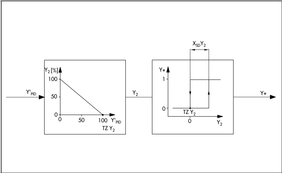
Fig. 42 · On-off output selected via C5-4
