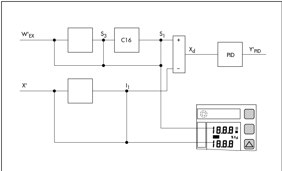
Fig. 78 · Digital displays in synchro control mode
