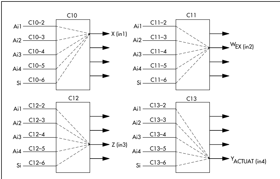
Fig. 2 · Assignment of analog inputs
